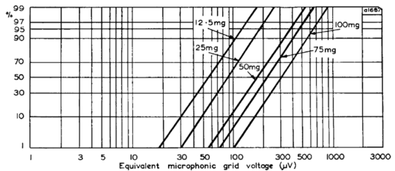
Fig. 3—Cumulative distribution characteristics of EF86 valves
