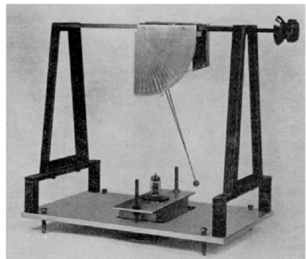
Fig. 6—Apparatus for measuring microphony by shock excitation
