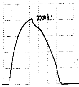
Figure 7. Measured current waveform for a 125A circuit-breaker when protecting a battery string within one of Telstra's distributed power supplies. 667A/div and 0.5ms/div.
