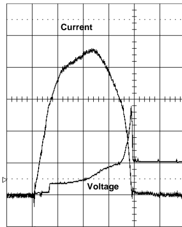
Figure 3. Measured current and voltage waveforms for a 125A circuit-breaker operating in 54VDC test circuit with about 12kA prospective current and about 1ms prospective time constant; 1kA/div current, 50V/div voltage and 0.5ms/div.
