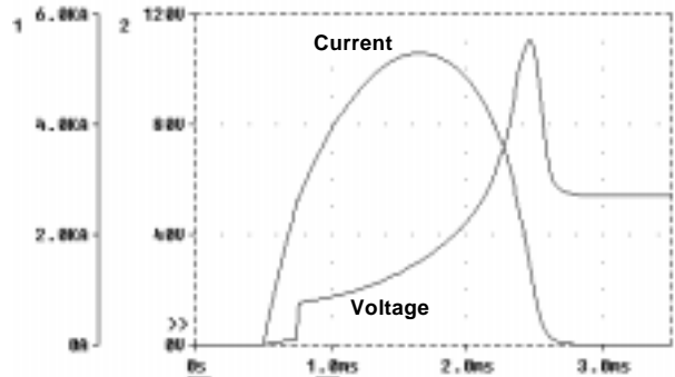
Figure 6. Simulated current and voltage waveforms for a 125A circuit-breaker operating in 54VDC circuit with 12kA prospective current and 1ms prospective time constant.
