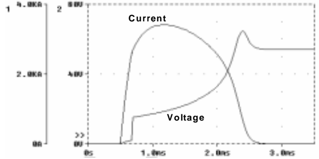
Figure 5. Simulated current and voltage waveforms for a 125A circuit-breaker operating in 54VDC circuit with 5.2kA prospective current and 0.25ms prospective time constant.
