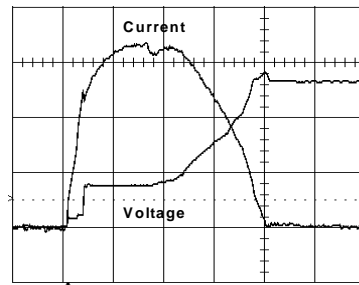
Figure 2. Measured current and voltage waveforms for a 125A circuit-breaker operating in 54VDC test circuit with 5.2kA prospective current and 0.25ms prospective time constant; 1kA/div current, 20V/div voltage and 0.5ms/div.
