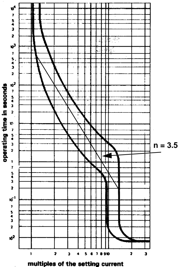
Figure 1. 125A circuit-breaker current-time operating boundary curves (courtesy of GEC ALSTHOM AUSTRALIA).
