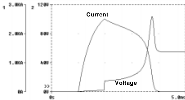
Figure 8. Simulated current and voltage waveforms for a 125A circuit-breaker when protecting a battery string within one of Telstra's distributed power supplies.
