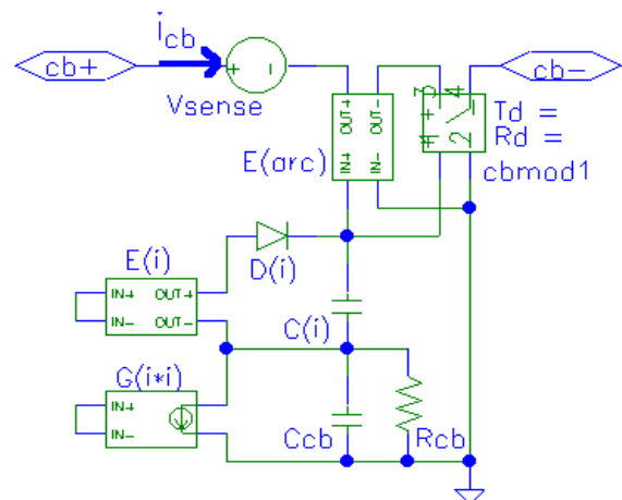
Figure 4. Circuit-breaker model.
